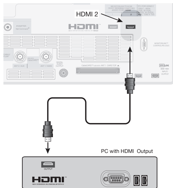
Figure 1. Connecting a Computer with an HDMI Monitor Output
